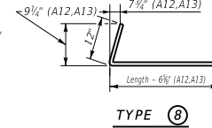
Reinforcement Details
